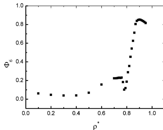
FIG. 7. The 2D bond order parameter \Phi_6 as the function of density for the SW molecules confined in a cylindrical hard pore of D=2.2 at T=1.0 and the potential range \lambda=1.2 .
