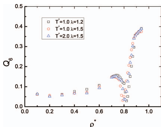
FIG. 6. The bond order parameter Q_6 as the function of density for the SW molecules confined in a cylindrical hard pore of D=2.2 at different temperature and potential range. Symbols square, circle and triangle represent system at T=1.0 and \lambda=1.2 , T=1.0 and \lambda=1.5 , T=2.0 and \lambda=1.5 , respectively.
