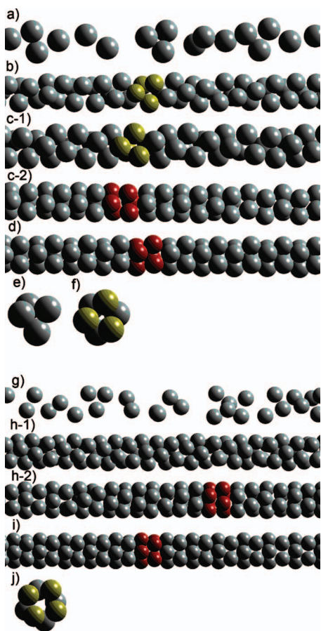
FIG. 10. Snapshots for the SW molecules confined in the narrow cylindrical pores of D=2.2 (a to d), and D=2.5 (g to i) at different average densities: a, \rho=0.3 (dilute fluid), b, \rho=0.75 (dense fluid, spiral packing of tetrahedron), c, \rho=0.85 (fluid-solid coexistence), d, \rho=0.92 (solid, triangular packing), g, \rho=0.3 (dilute fluid), h, \rho=0.85 (fluid-solid coexistence) and i, \rho=0.95 (solid, square packing). The tetrahedral, triangular, and square packings are shown in e, f, and j, respectively. Two different structures are found in the corresponding coexistence densities in D=2.2 (c-1 and c-2) and D=2.5 (h-1 and h-2).
