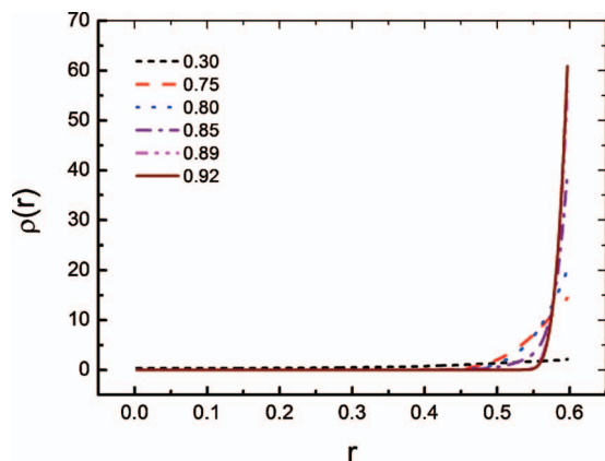
FIG. 9. Radial density profiles \rho(r) for the same system as in Fig. 8.
