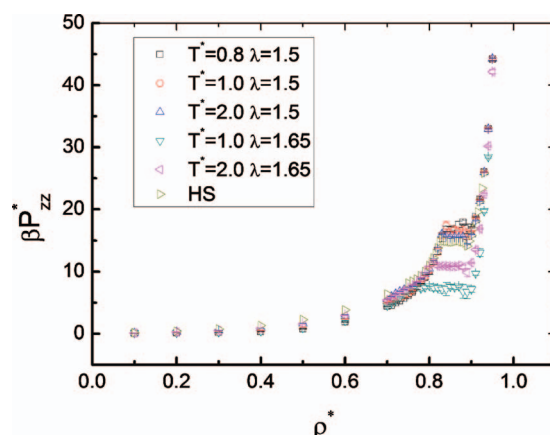
FIG. 5. The same equation of state as in Fig. 3 for D=2.5 and \lambda=1.5 at T=0.8, 1.0 , and 2.0 , \lambda=1.65 at T=1.0 and 2.0 . The equation of state of hard spheres confined in D=2.5 is shown for comparison.
