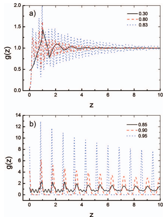
FIG. 11. Axial pair distribution function g(z) for the SW molecules confined in cylindrical pore of D=2.5 at T=1.0 and \lambda=1.5 , at different average densities, 0.30 (dilute fluid), 0.80 (dense fluid), 0.83 (around freezing density), 0.85 (within fluid-solid coexistence), 0.90 (around melting density), and 0.95 (solid).
