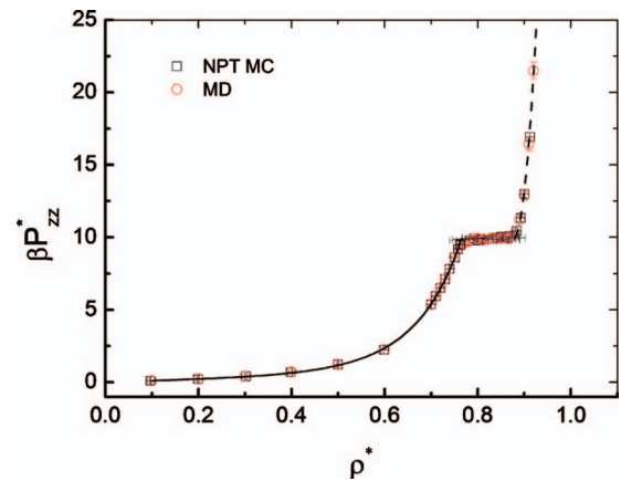
FIG. 1. Comparison of the equation of state ( \beta P_{zz}^* vs \rho^* ) of the SW molecules of \lambda=1.5 confined in cylindrical hard pore of D=2.2 at T=1.0 obtained by NPT MC and MD simulations, which are represented by square and circle symbols, respectively. The solid line indicates the fit of result at fluid branch using Eq. (1), and the dash line is the second order polynomial fit to the solid branch. Error bars are the standard deviation of 5 independent runs.
